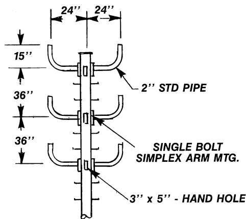
TENON ARM SLIPFITTER
