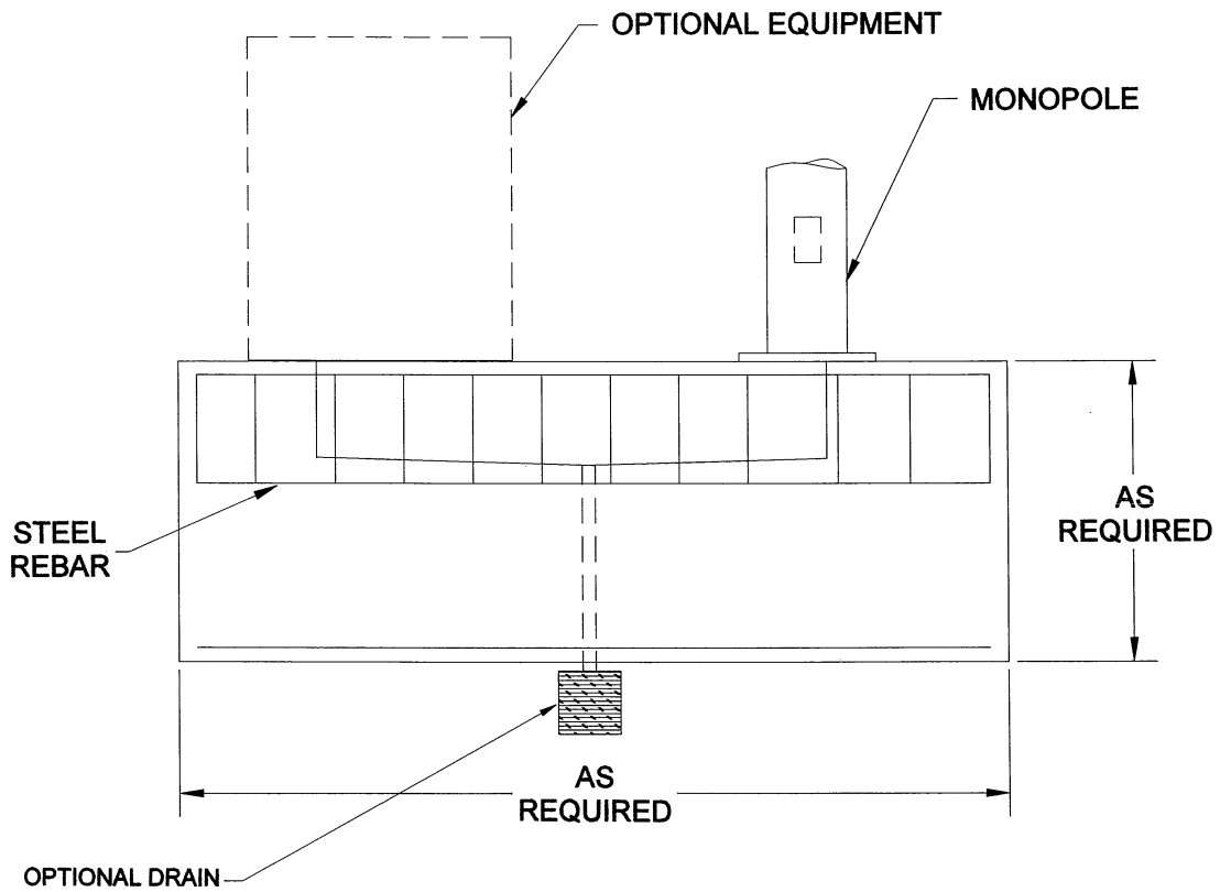
SPREAD FOOTING
