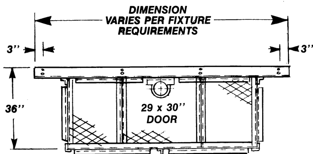
CAGE CONFIGURATION
