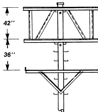
ANGLE FRAME WITH STAND-BAR
