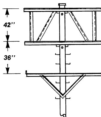
ANGLE FRAME WITH STAND-BAR
