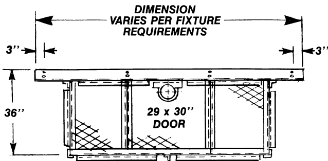
CAGE CONFIGURATION
