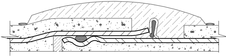
Gasketed Field Joints
