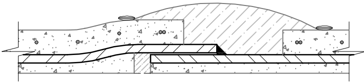
Lap Welded Field Joints
