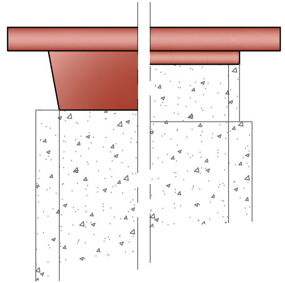
Flanged Ends
