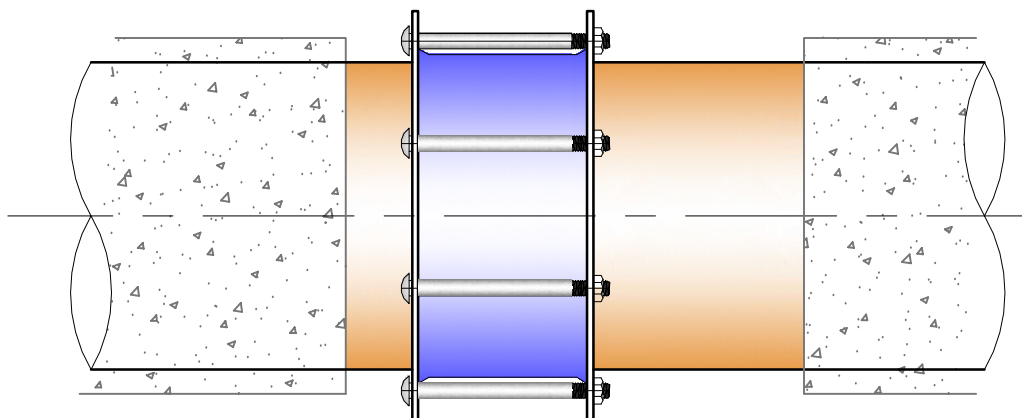
Bolted Couplings Sleeve & Grooved Type
